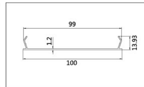
名称: 100 封盖 壁厚: 1.2mm
