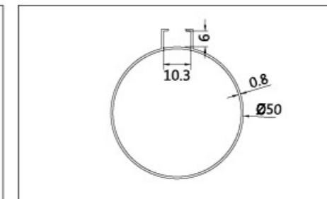
名称: 50x0.8TH 壁厚: 0.8 1.0 1.1mm
