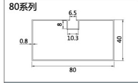
名称: CD-40x80TH 壁厚: 0.8mm
