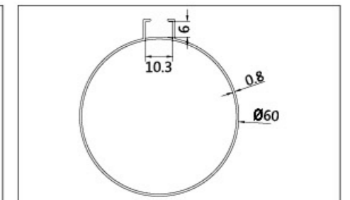
名称: 60x0.8TH 壁厚: 0.8 1.0mm
