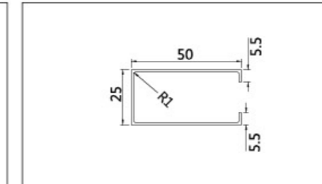
名称: 25x50UC 壁厚: 0.6 0.7 0.9 mm
